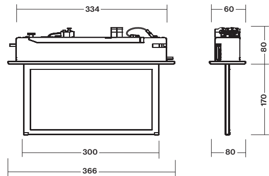
C.LEDLUX-V / MULTILED-V Dimensions
